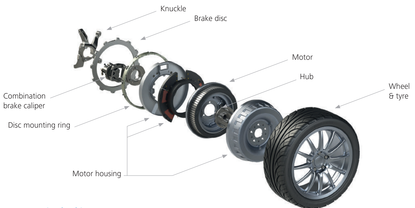
Regenerative braking system
